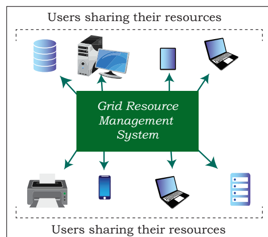
Figure 3.13: Grid computing
