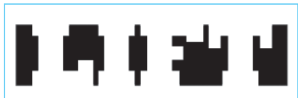
Fig.5.12 : Surroundedness
