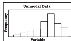
Unimodal Data
